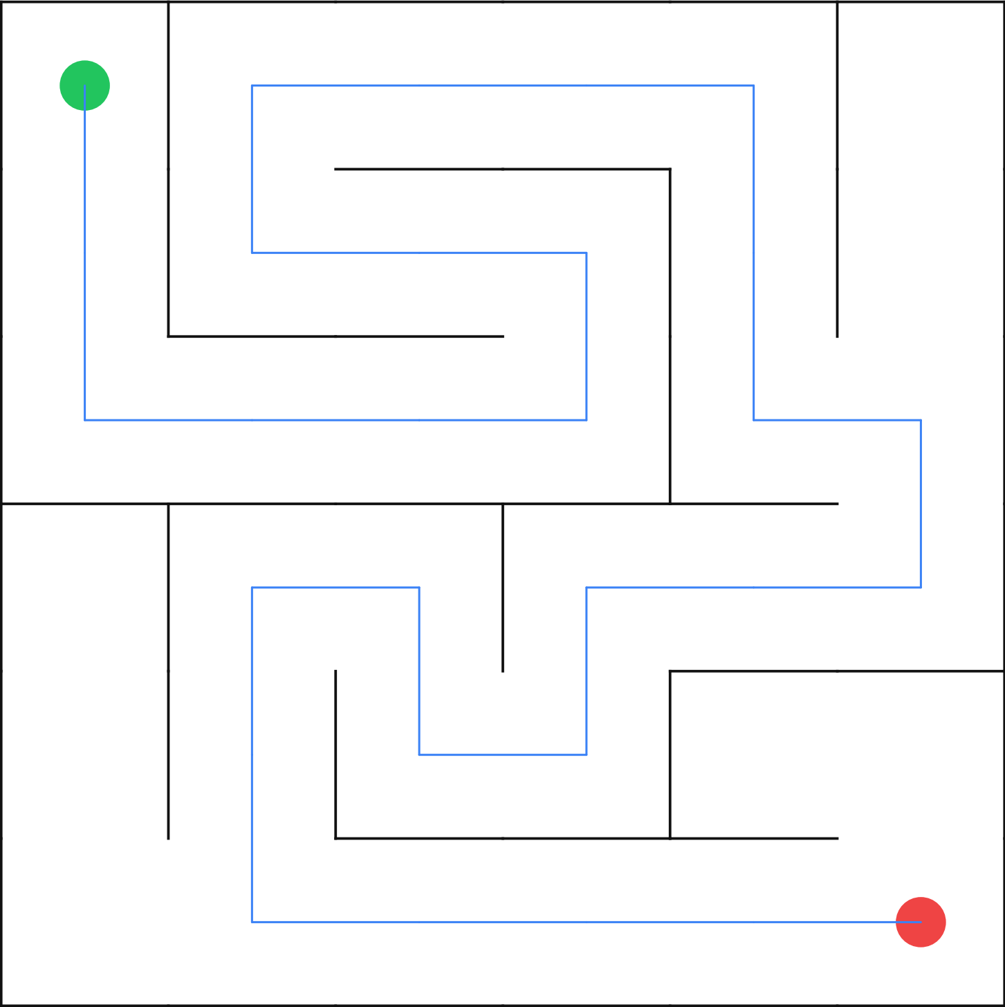
Maze 6×6 — seed 33524140
