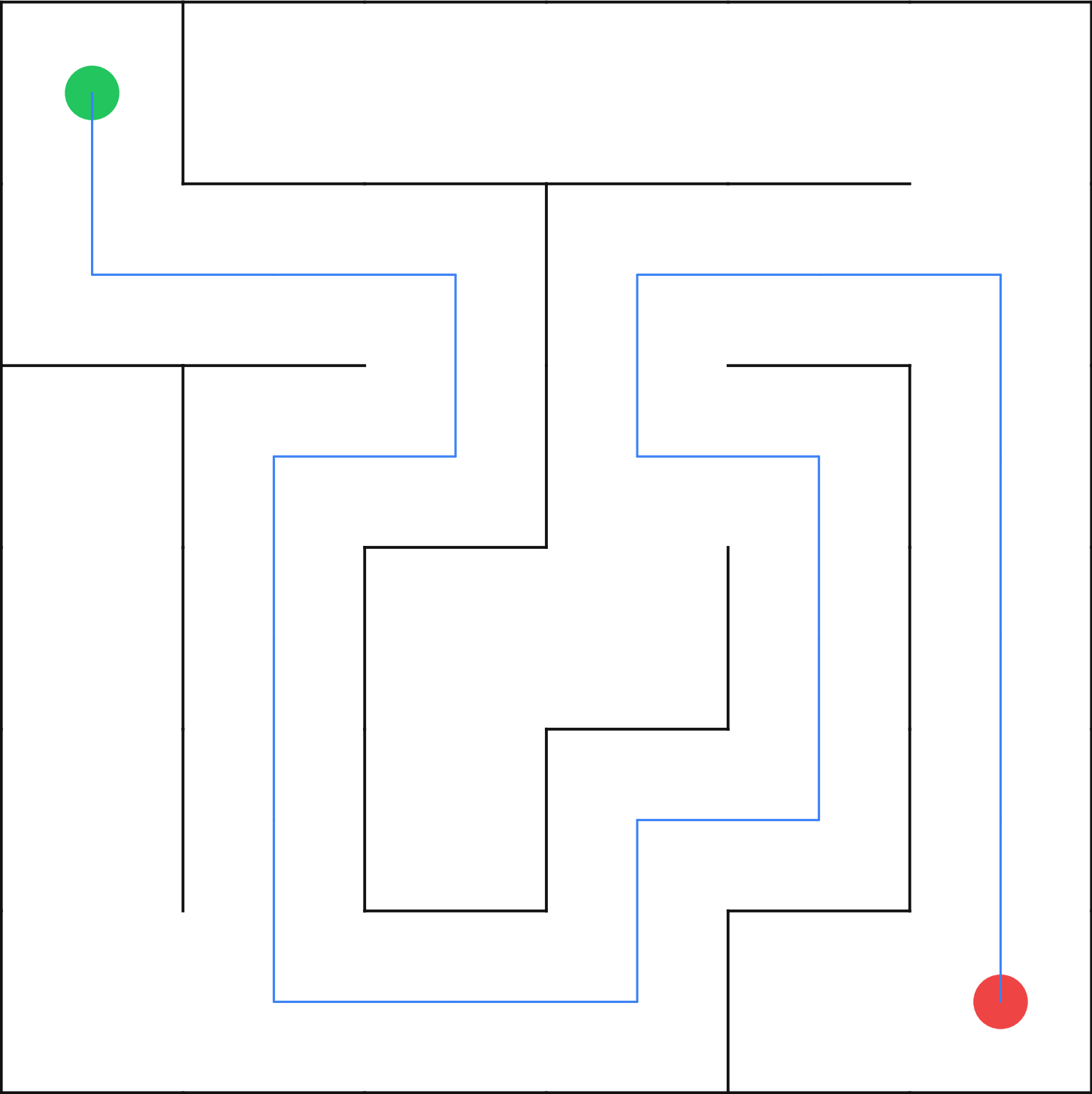
Maze 6×6 — seed 134686680
