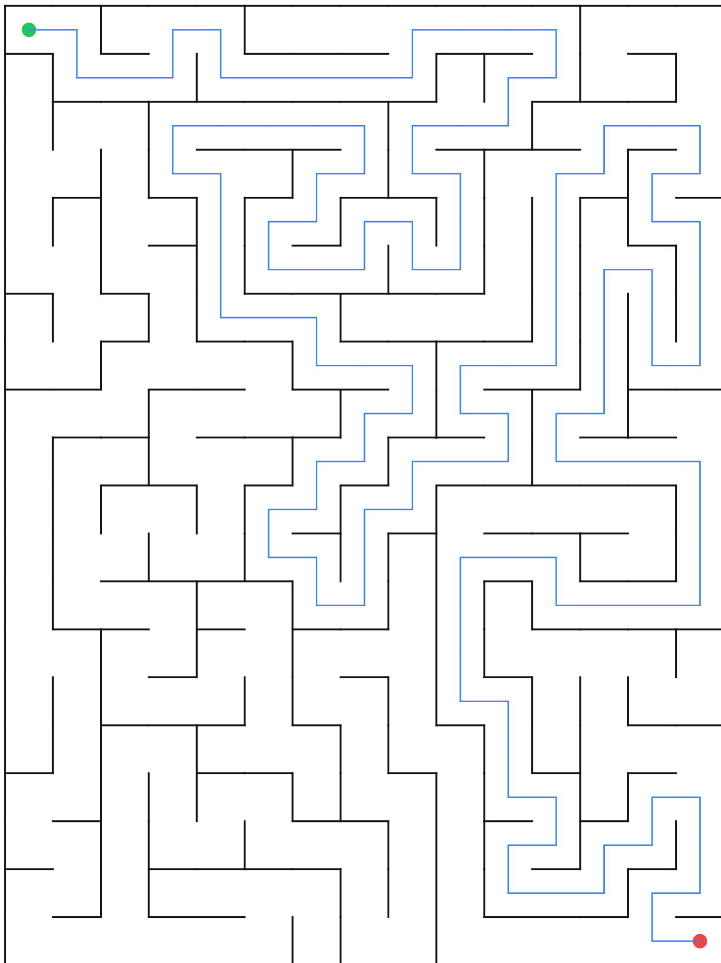
Maze 15×20 — seed 835041835
