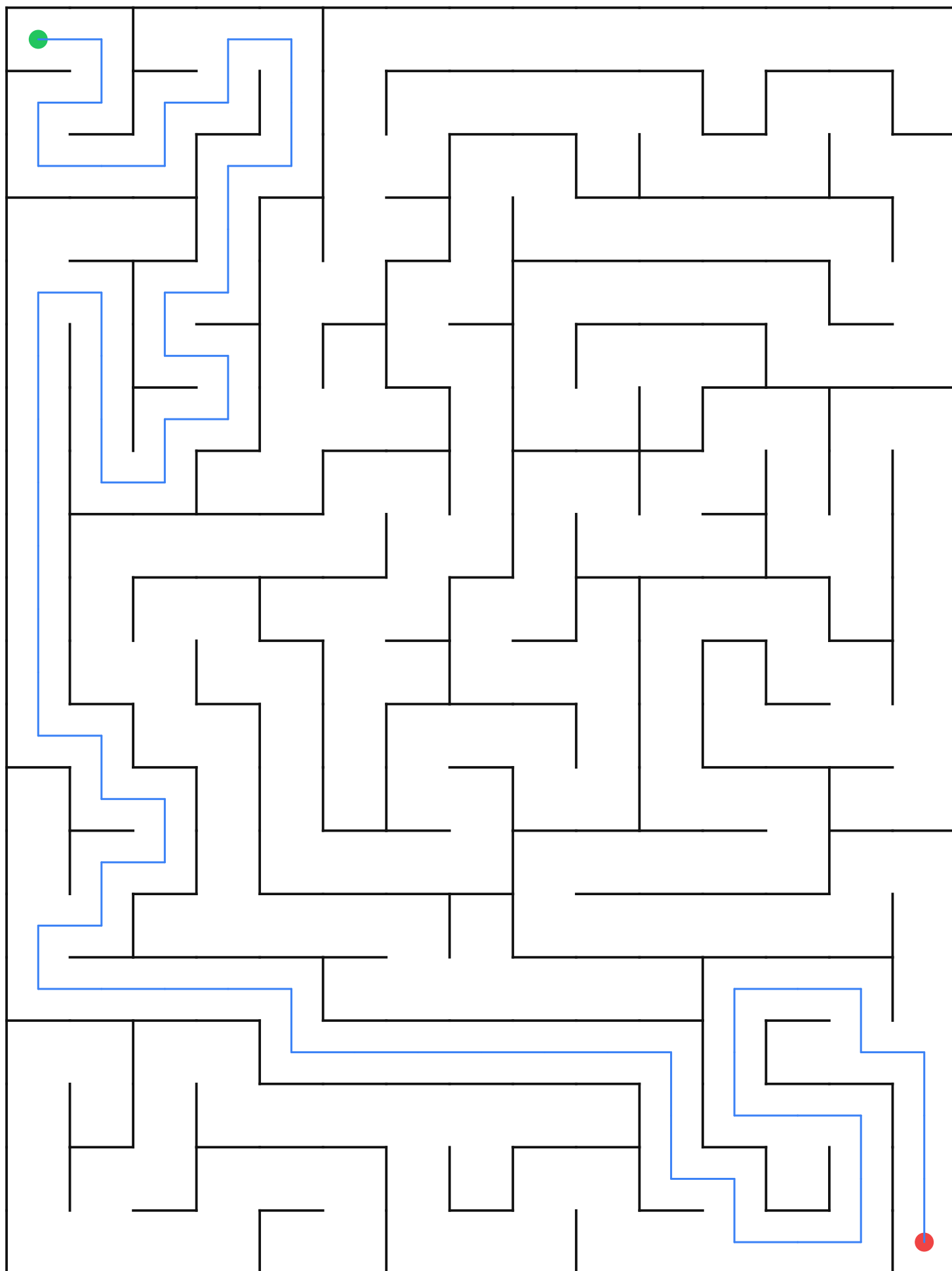
Maze 15×20 — seed 3382398394
