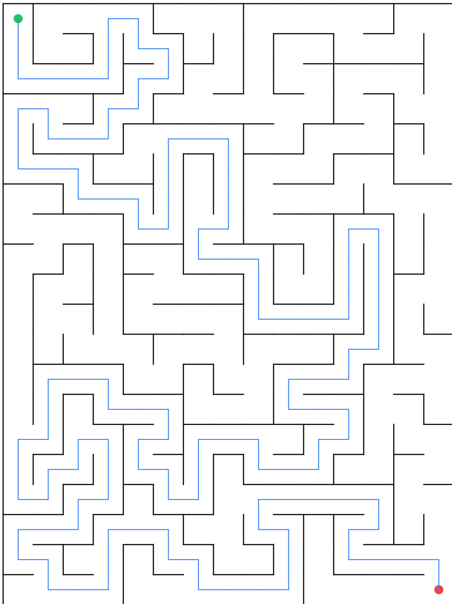
Maze 15×20 — seed 3029373063
