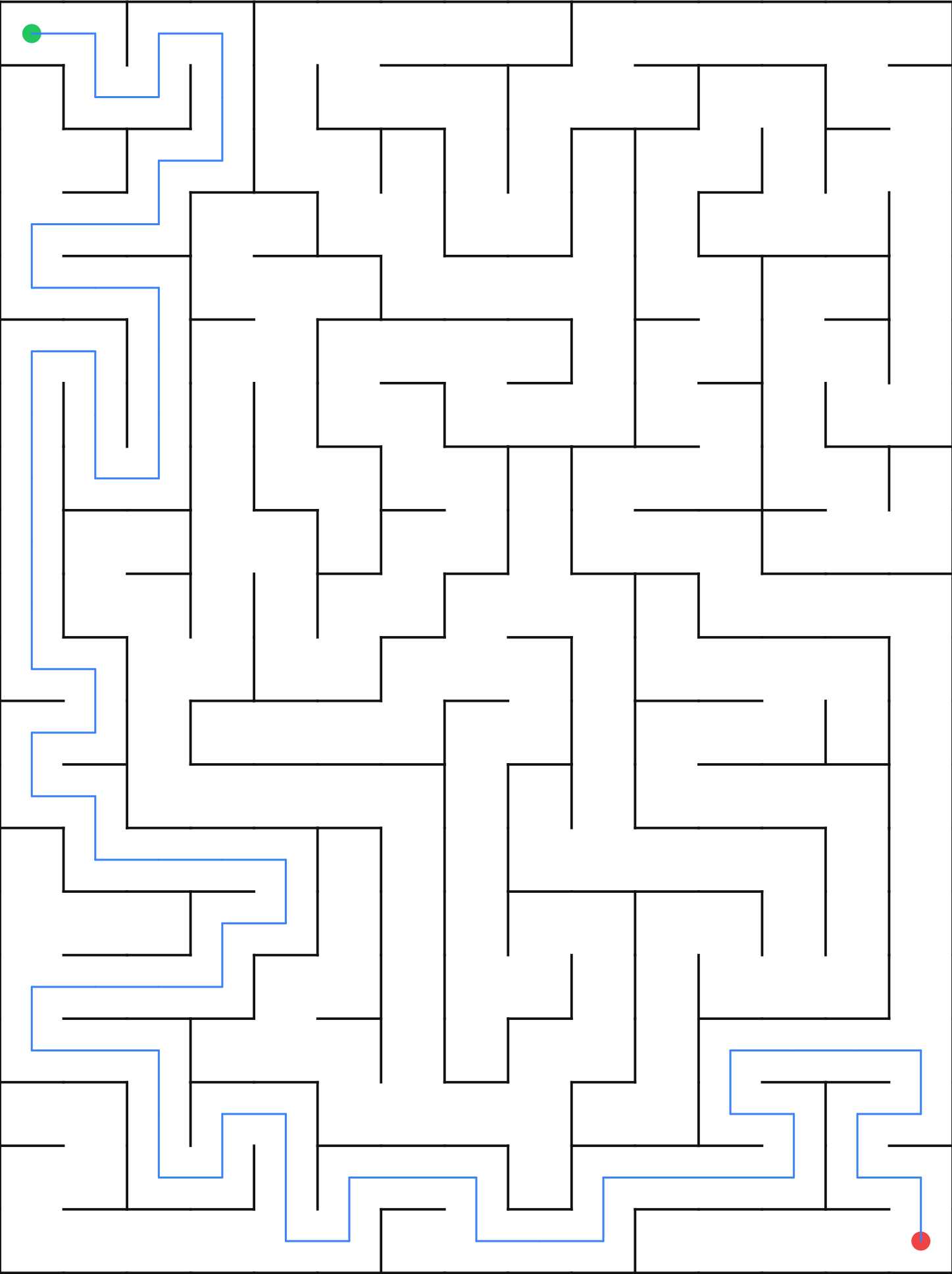
Maze 15×20 — seed 2208525334
