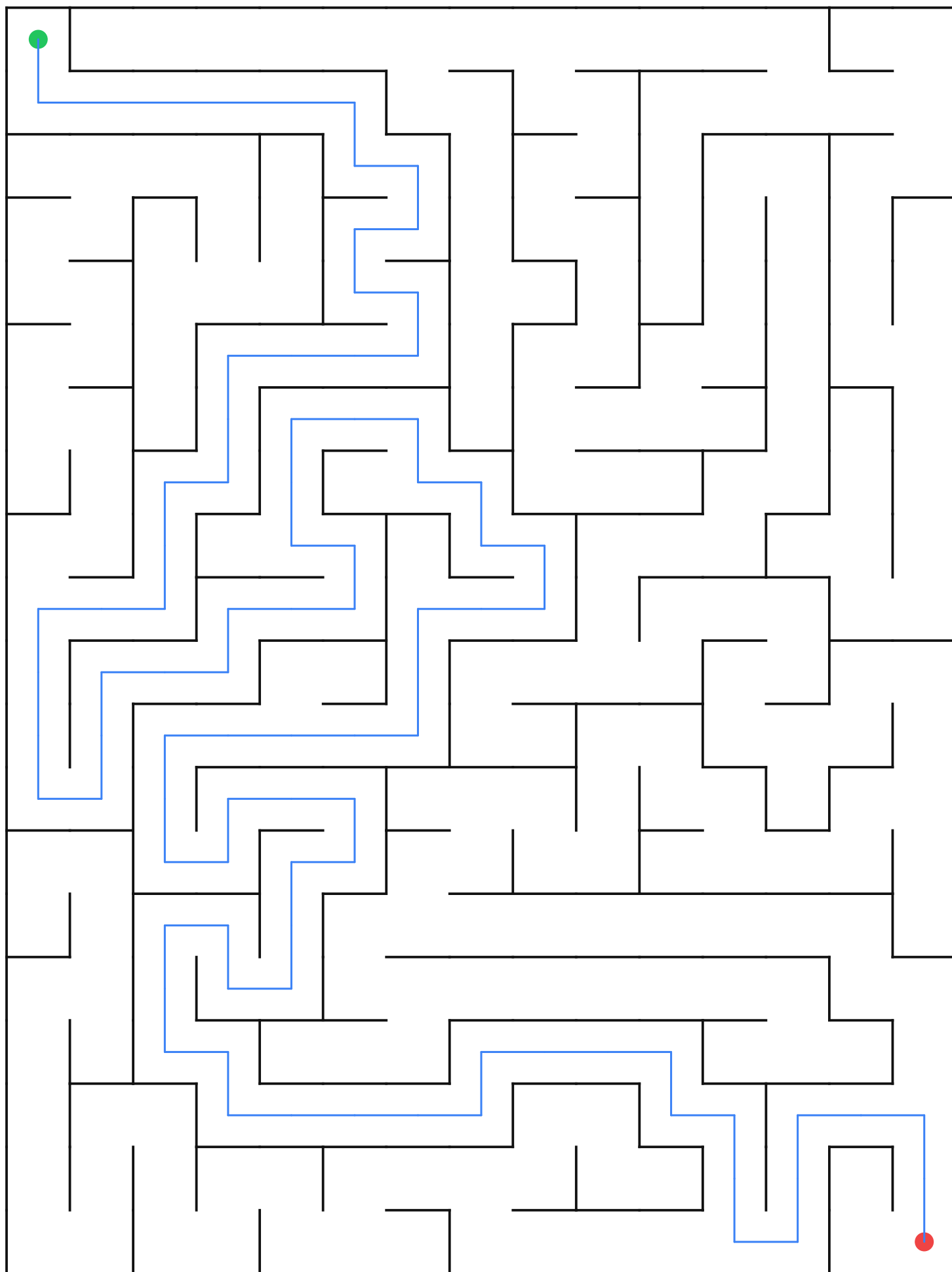
Maze 15×20 — seed 2148415001
