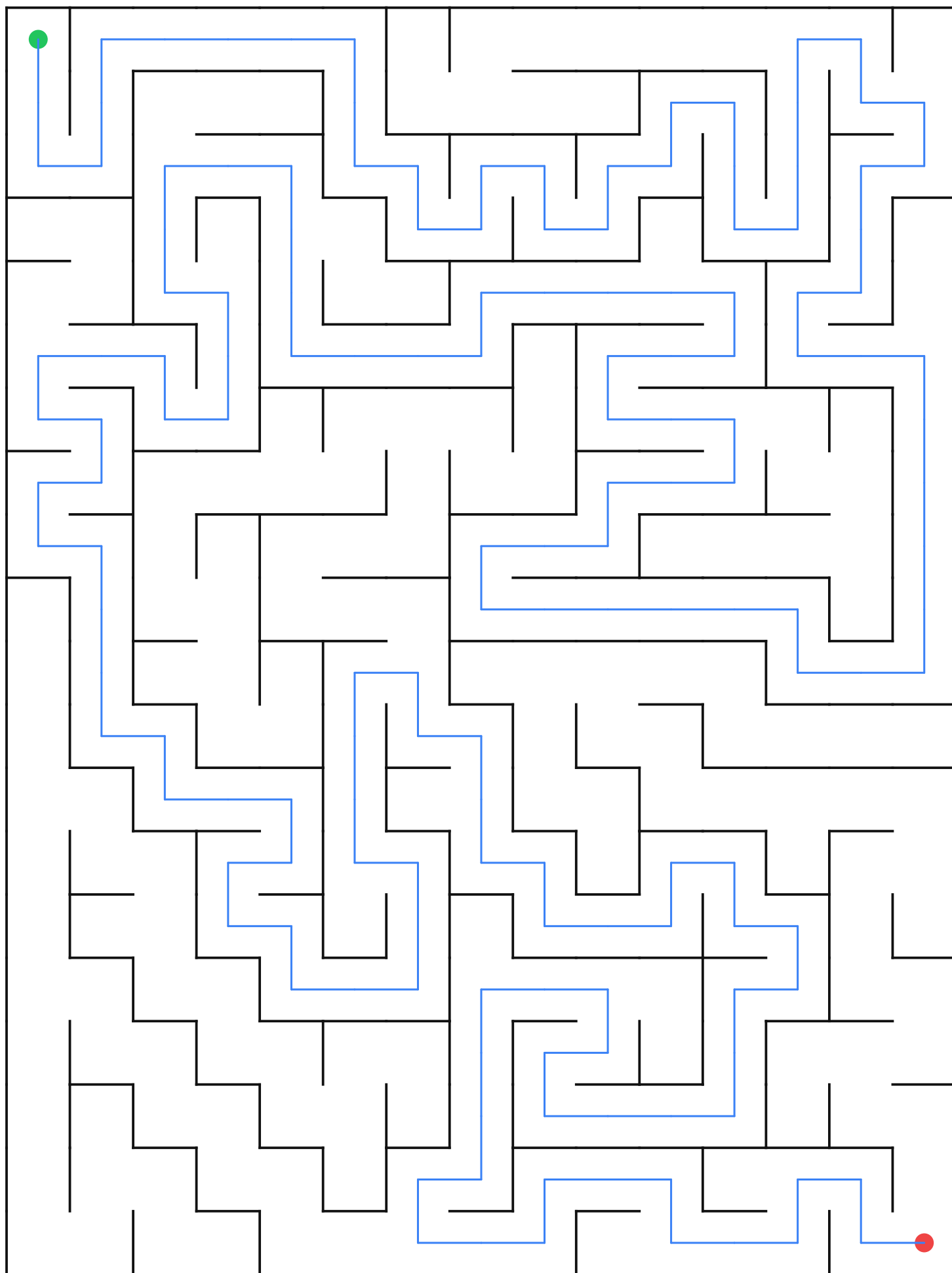
Maze 15×20 — seed 2101043507
