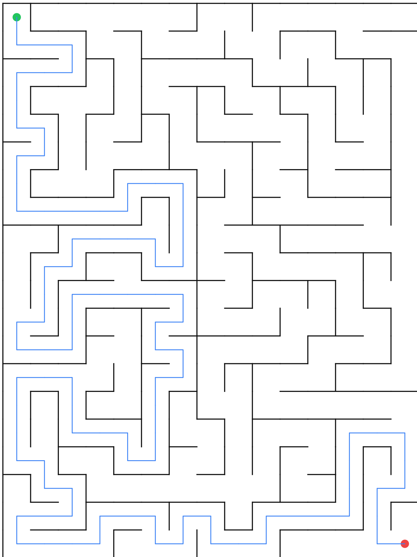
Maze 15×20 — seed 1922218565
