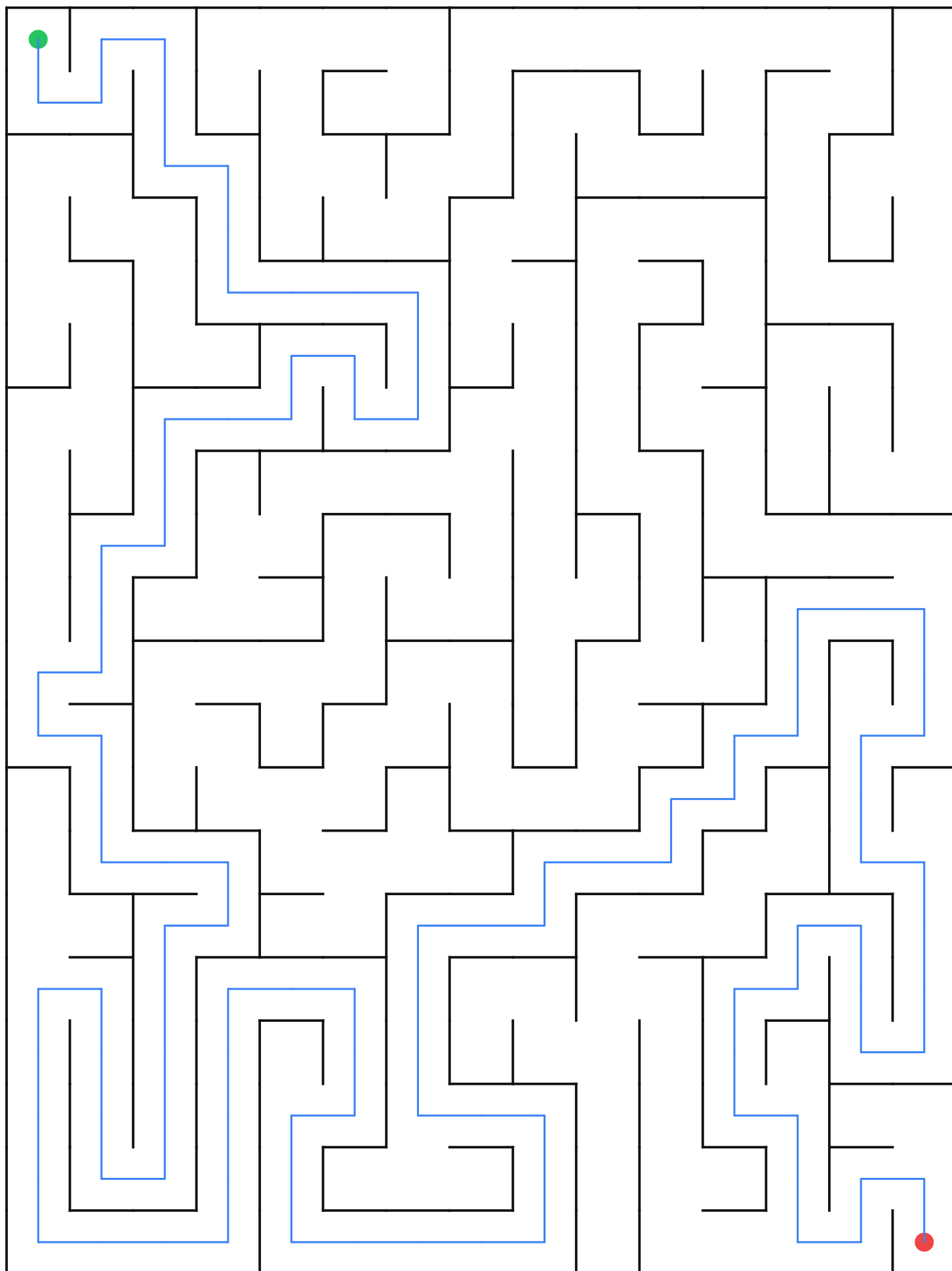
Maze 15×20 — seed 1624697213
