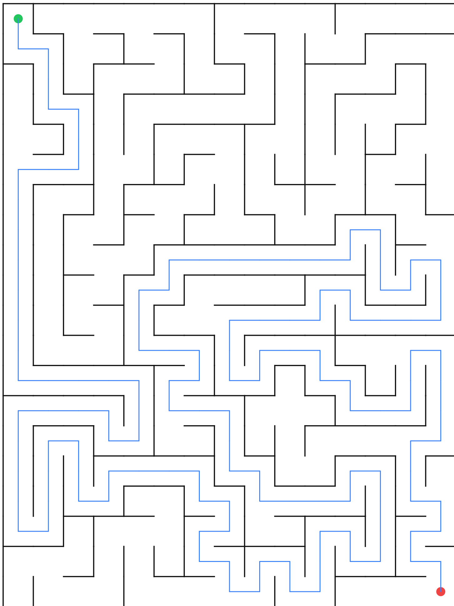
Maze 15×20 — seed 1216931787
